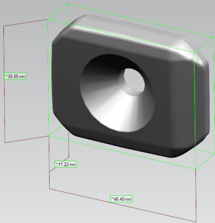
Buckle
