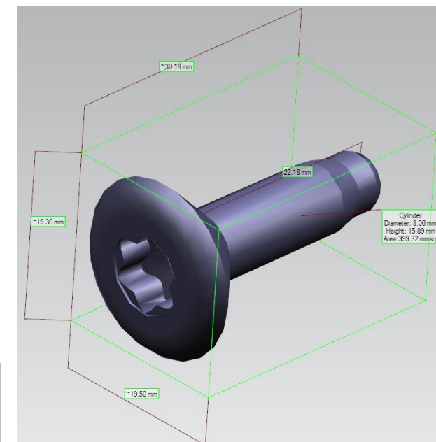
Fastener
